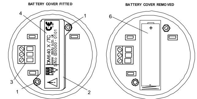
Fig 2 Rear view
