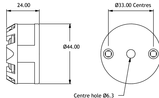
Figure 1 (All dimensions in mm)
