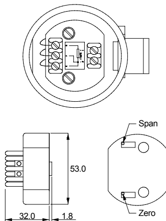
Mounting holes: 2 holes 4.5mm diameter, 33mm centres
